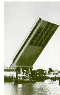
the Miller-Sweeney bascule bridge on Alameda Island
